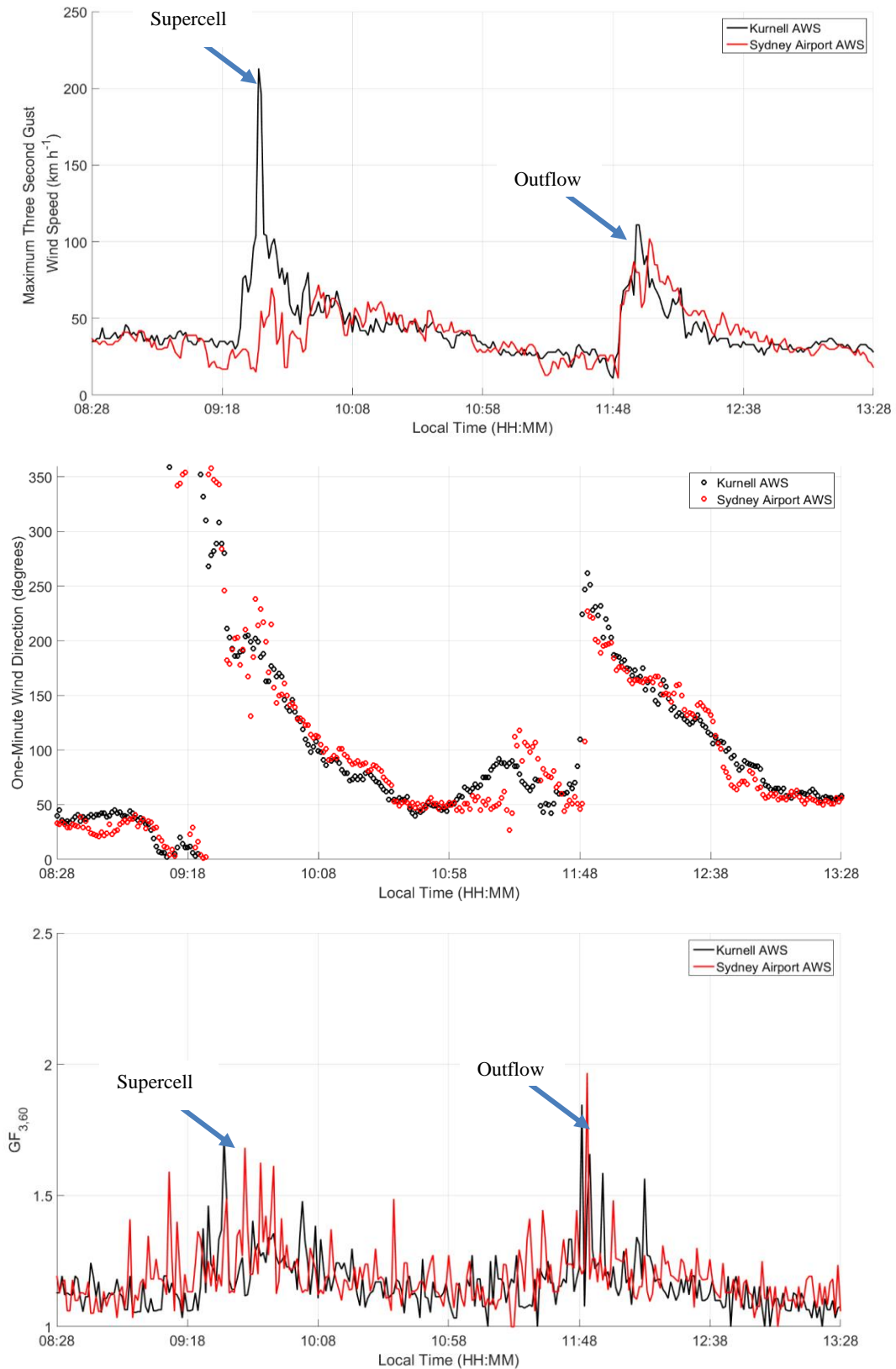
Figure 2. Kurnell (solid black line) and Sydney Airport (solid red line) AWS station maximum three-second gust wind speed time histories (upper), wind direction (middle) and gust factor ( G_{3,60} ) (lower), during the passage of a tornadic supercell and thunderstorm outflow.
