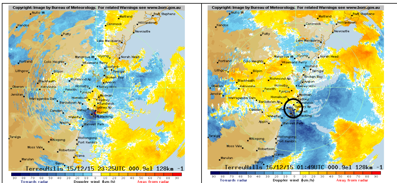
Figure 1. The 128 km 0.9o elevation PPI of Doppler radial velocity (km h -1 ) from the Terrey Hills Doppler radar at 09:25 (left) and 11:49 (right) on 16 December 2015. Cool colours represent inbound radial velocities towards the radar and hotter colours represent outbound radial velocities away from the radar. The thick red arrow in the left figure points to the folded radial velocities that exceeded the Nyquist velocity of the Doppler radar. The leading edge of the thunderstorm outflow winds is circled in black in the right image.
