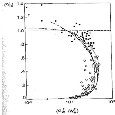
Figure 8. Vertical velocity variance under convection (Spillane, HESS 1988)
