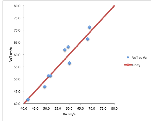
Figure 6. Tangential Velocity – modelled and measured
