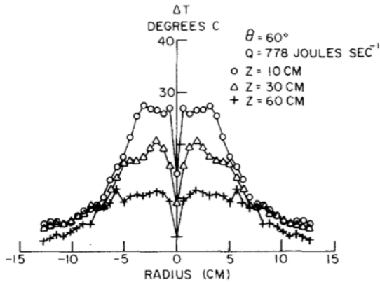
Figure 4. Scaled Temperature excess vs Radius, 60° vane angle, 778W (Mullen, Maxworthy 1977)
