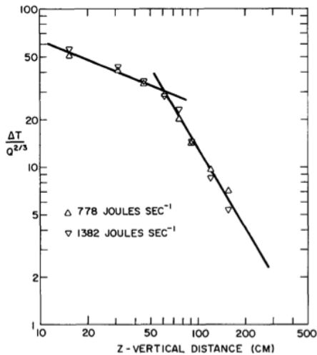
Figure 5. Scaled Temperature Excess vs Height (Mullen, Maxworthy 1977)
