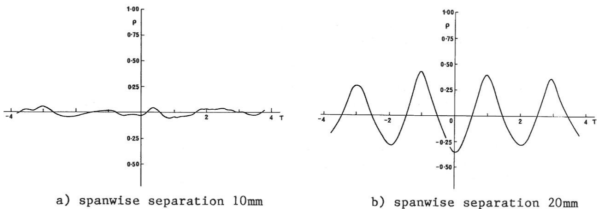
Fig.4 Mid-chord Cross-correlations
